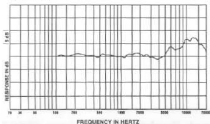
FIGURE 1 — Frequency Response
